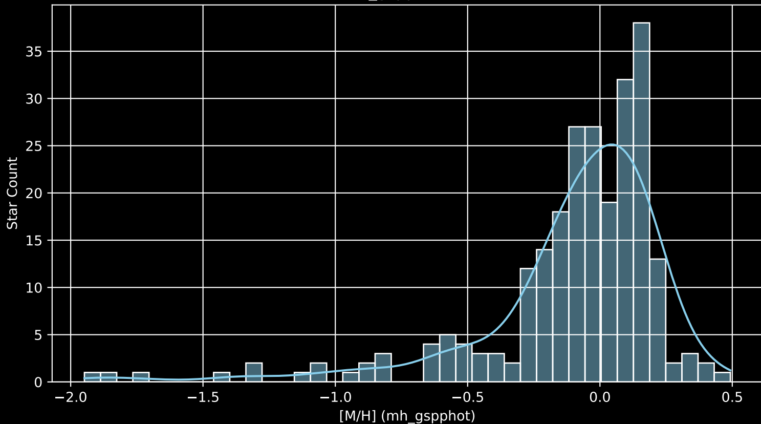
APOGEE DR17 Field: [079-06 [M/H] (mh_gspphot) (n= 244)
