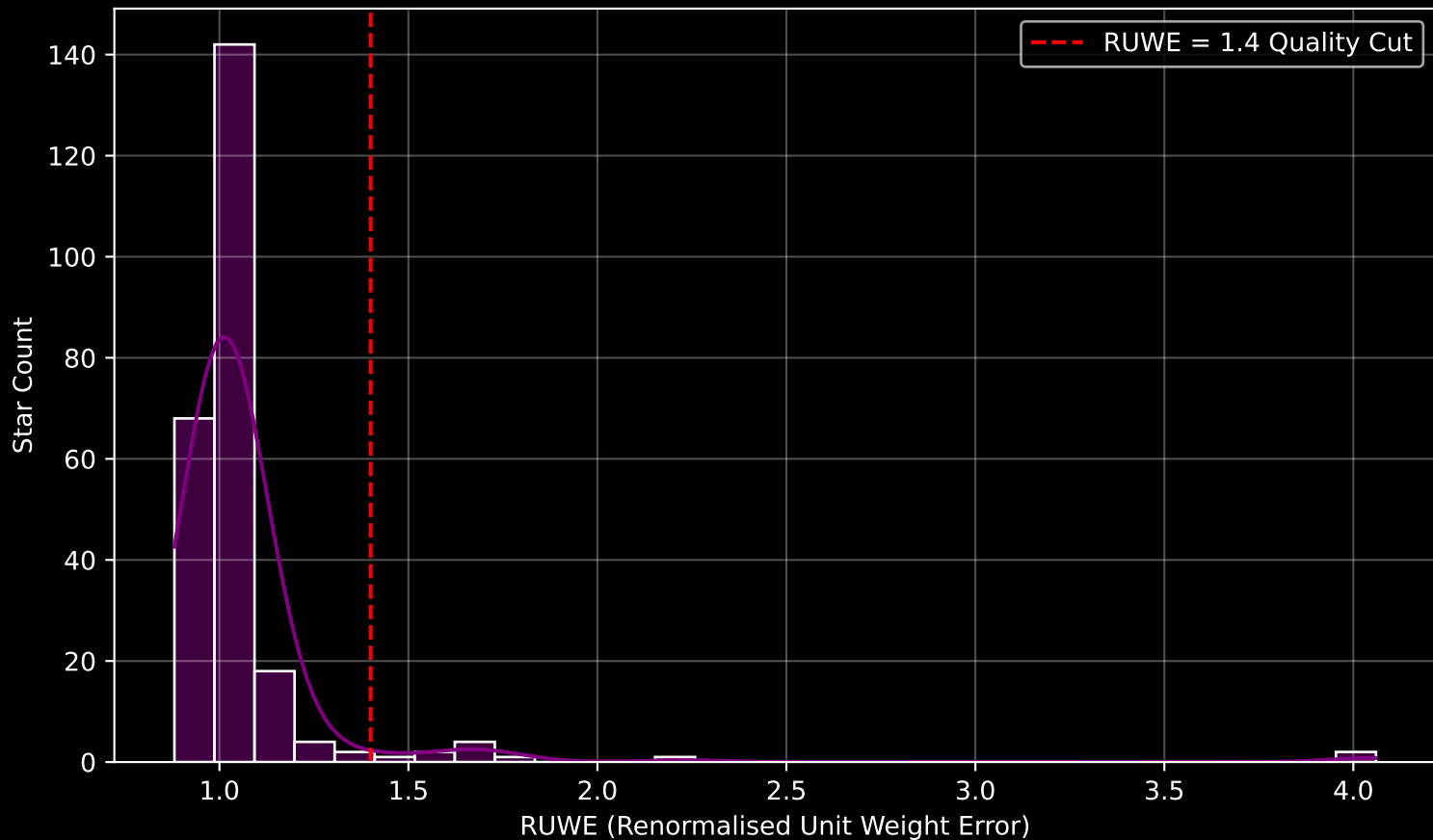
GAPOGEE DR17 Field [079-06] RUWE Distribution (n= 245)
