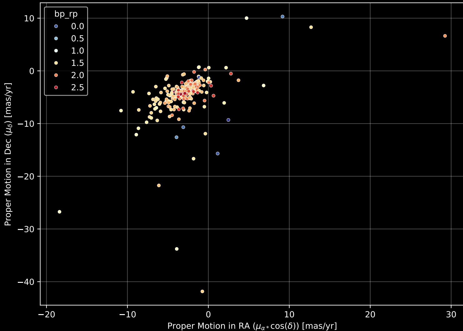
APOGEE DR17 Field: [079-06] Proper Motion Diagram (n= 246)
