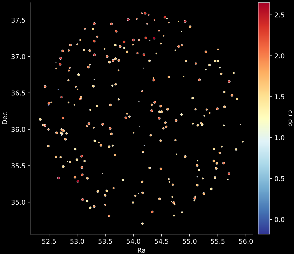
APOGEE DR17 Field: [079-06] Stars: 246
