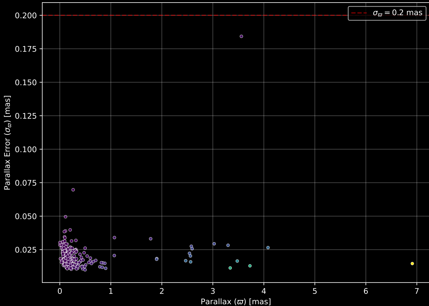
APOGEE DR17 Field: [079-06] Parallax Quality (n= 246)
