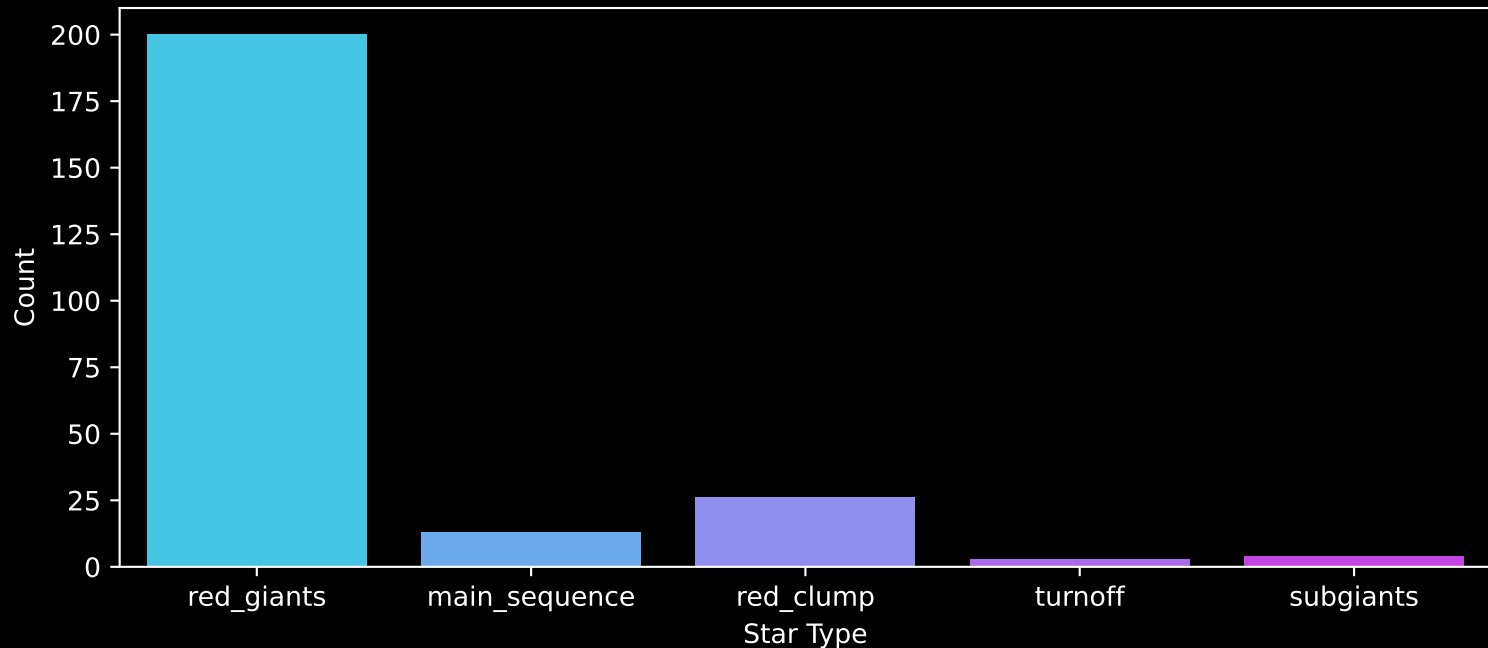
APOGEE DR17 Field: [079-06] Count plot of Star Type
